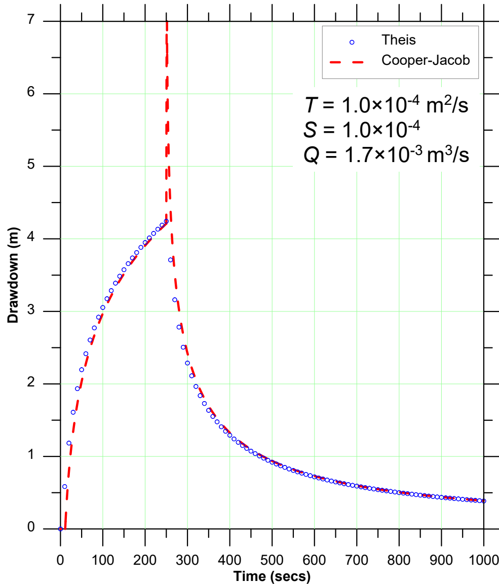
Figure 15. Theis solution and Cooper-Jacob approximation for Example 3
