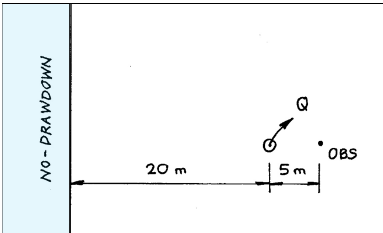
Figure 19. Conceptual model for pumping near an extensive surface water feature
