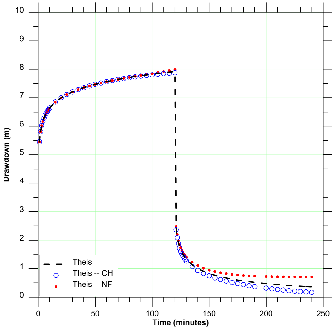
Figure 24. Calculated drawdowns during pumping and recovery
