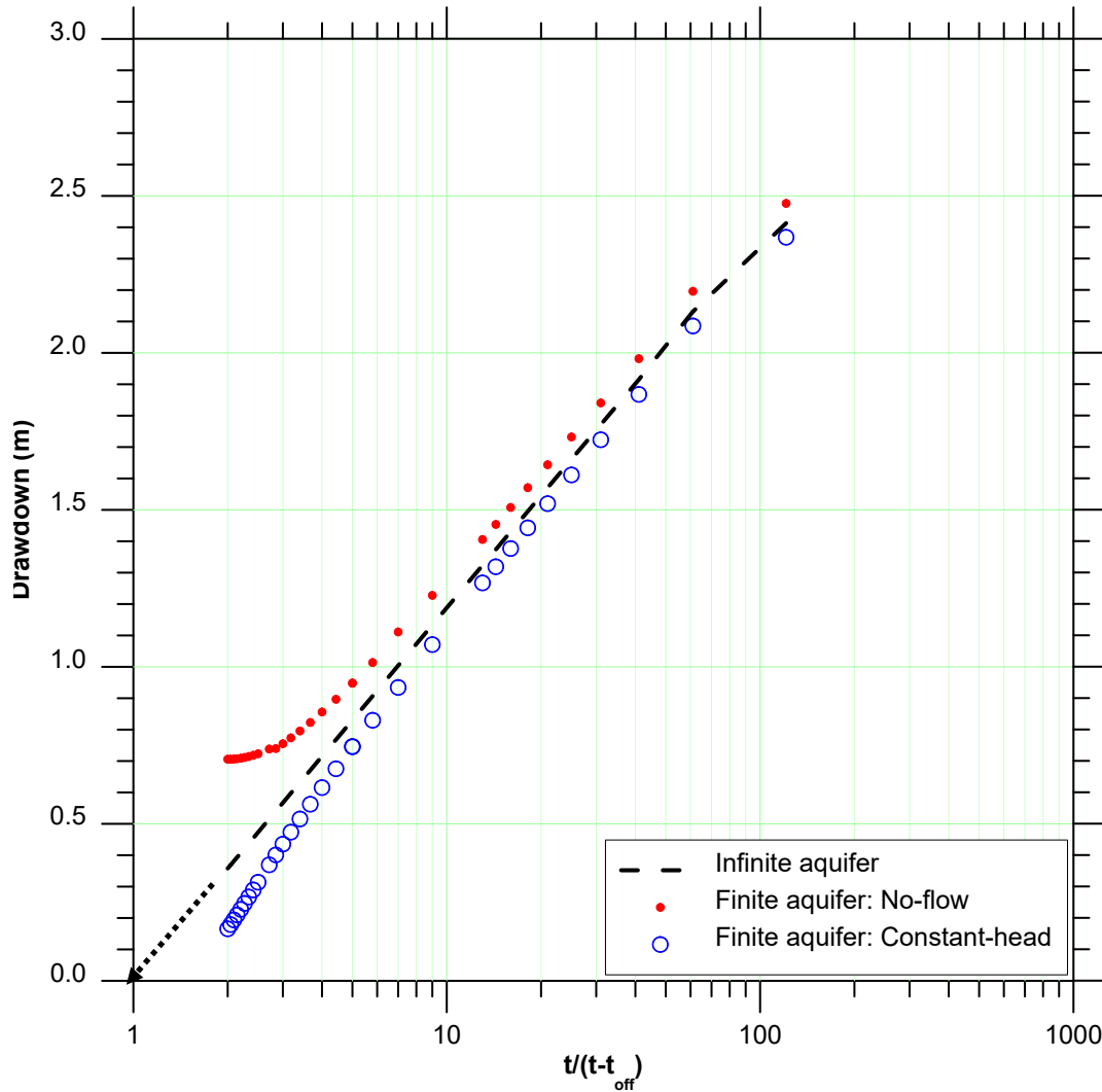
Figure 25. Semilog recovery plot
