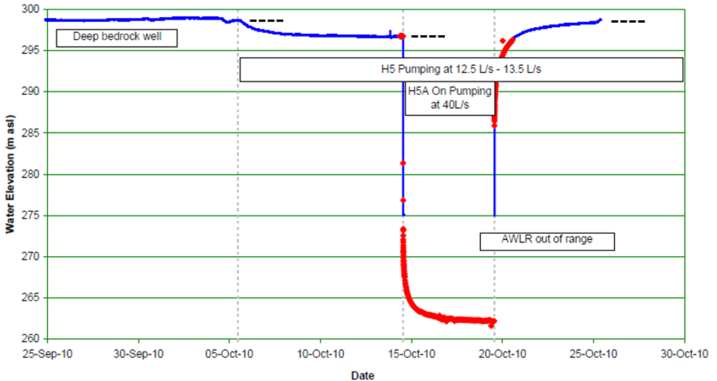
Figure 11. H5A pumping test - water levels in the pumping well
