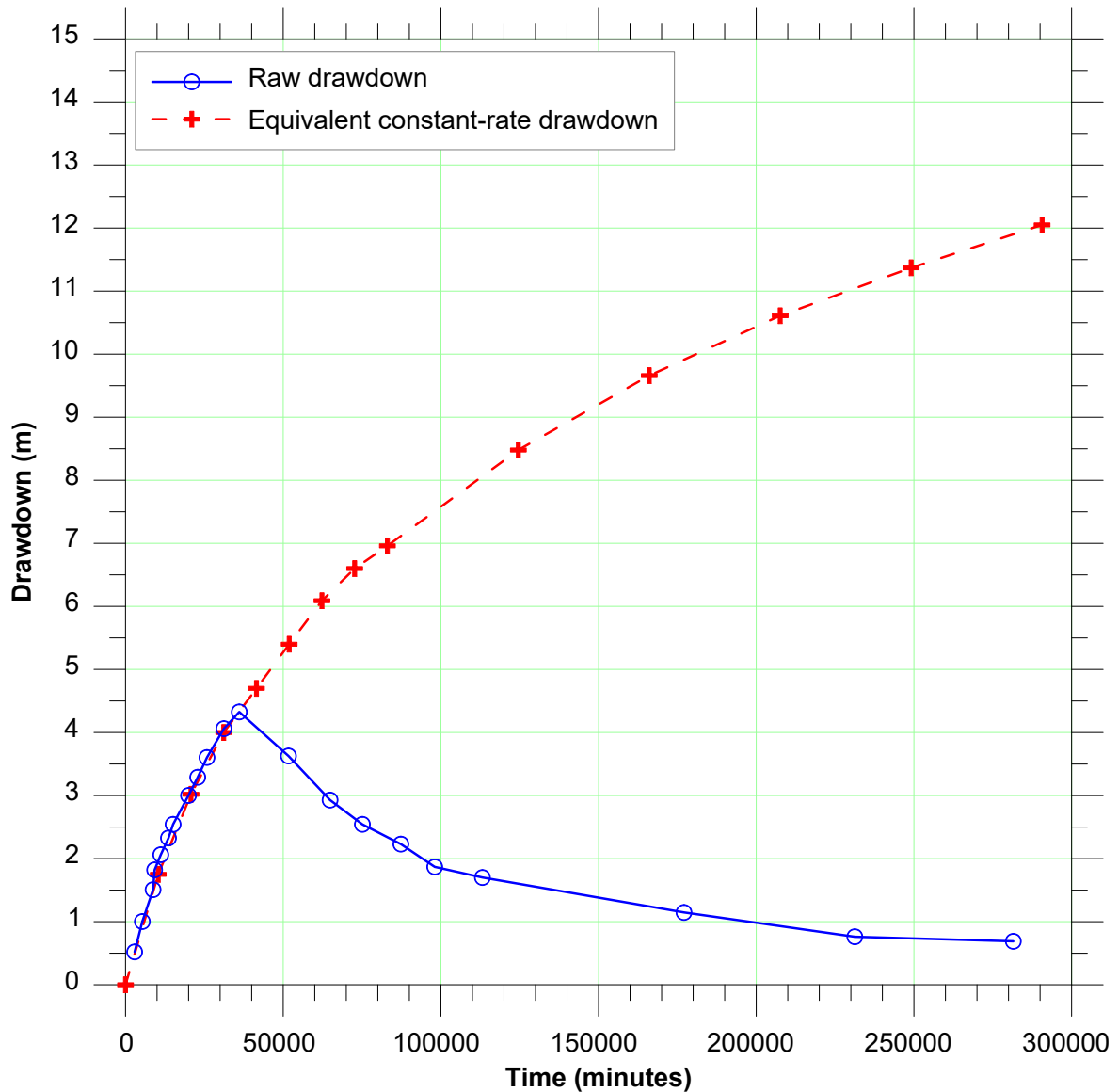
Figure 33. Complete record of equivalent constant-rate drawdowns
