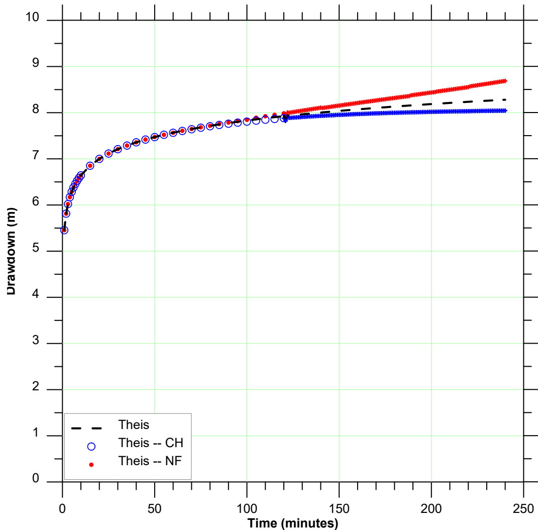
Figure 30. Equivalent constant-rate drawdowns
