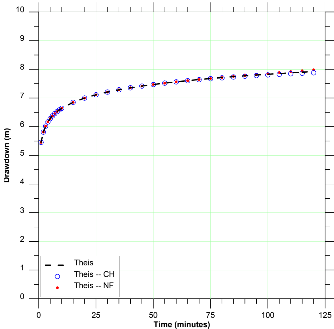
Figure 23. Calculated drawdowns during the pumping period
