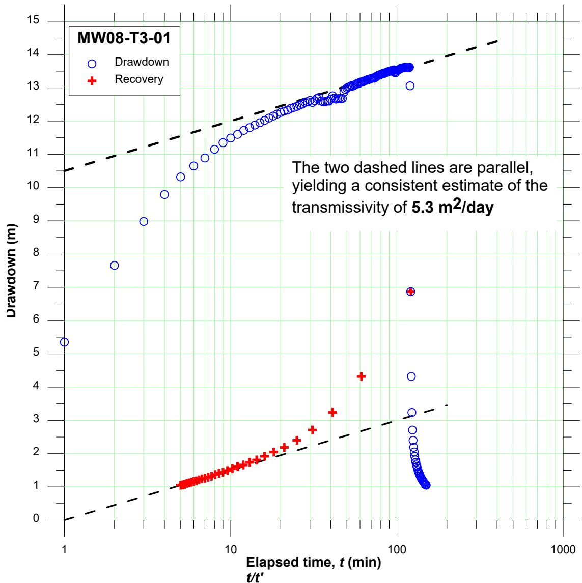
Figure 21. Example check on the consistency between the drawdown and recovery analyses
