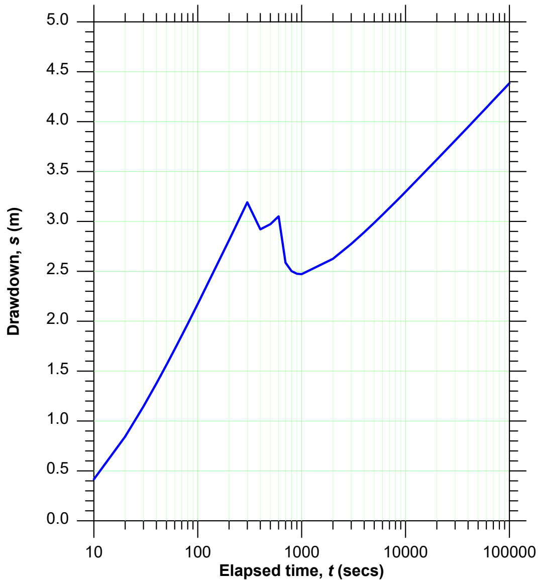
Figure 4. Drawdowns calculated at r = 5 m
