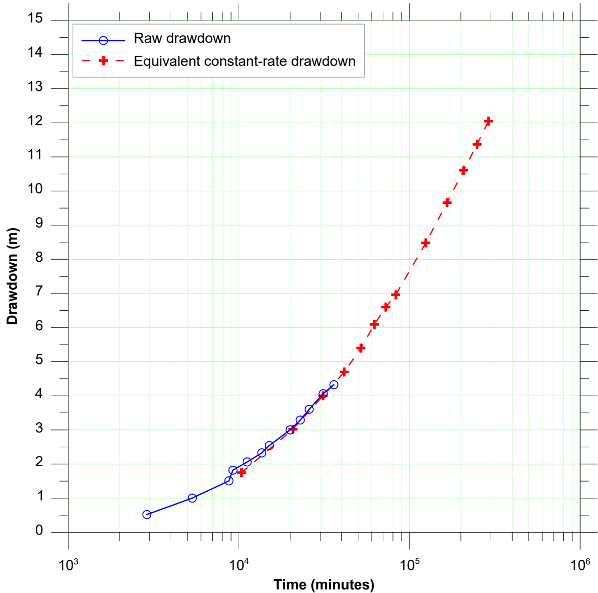
Figure 34. Semilog plot of equivalent constant-rate drawdowns
