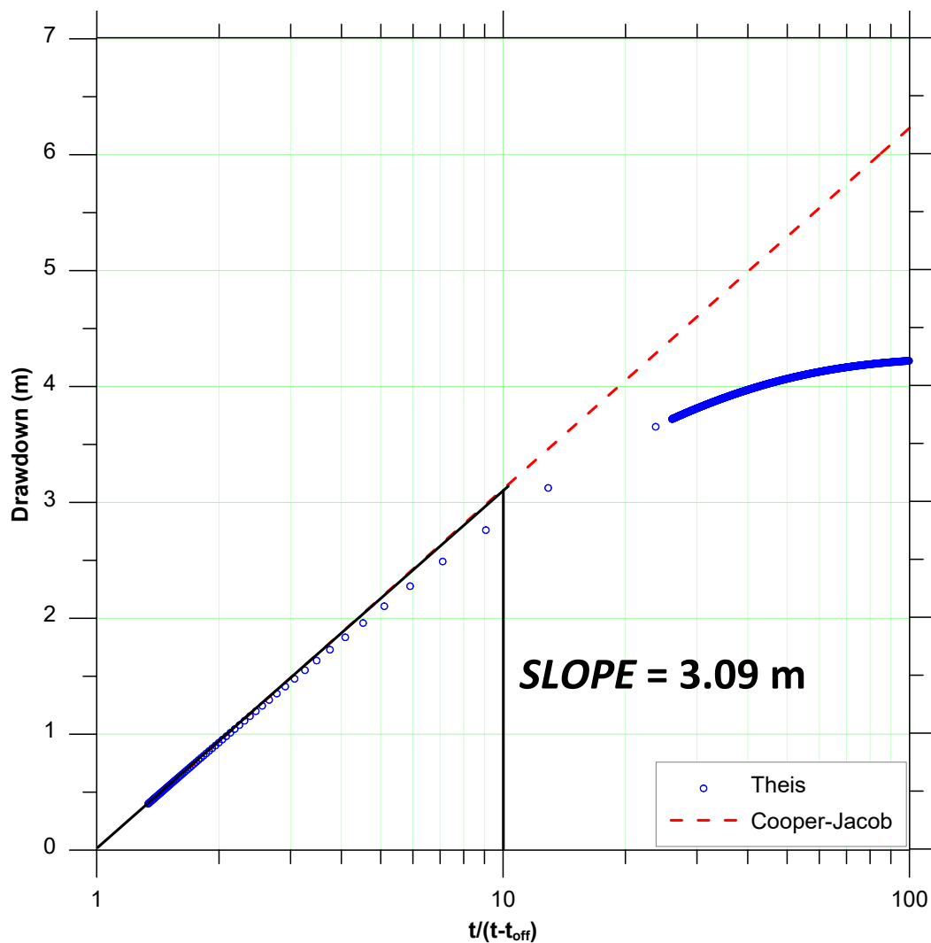
Figure 17. Straight-line recovery analysis
