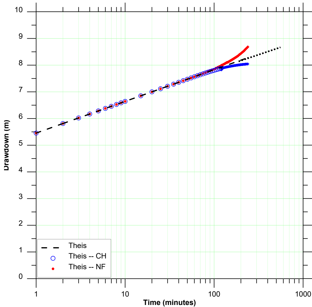
Figure 31. Equivalent constant-rate drawdowns, semilog plot
