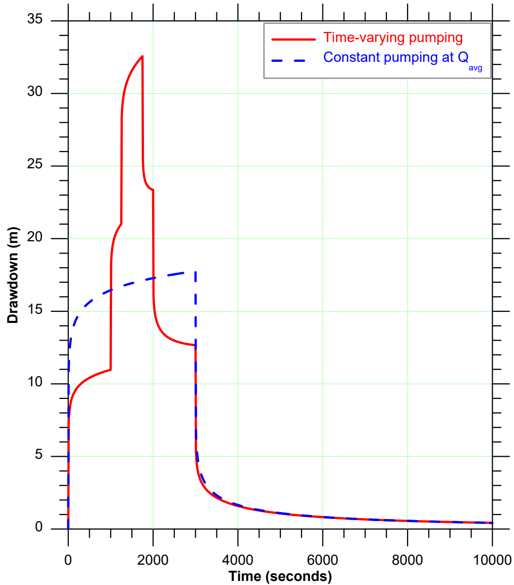
Figure 9. Drawdowns for the full duration of the pumping test
