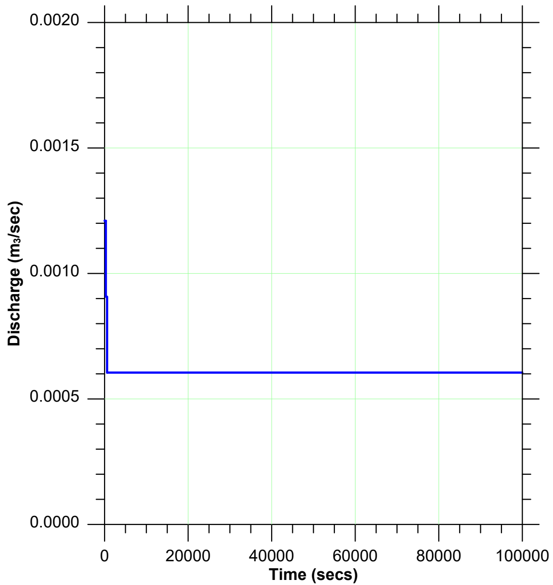
Figure 3. Pumping history for Example 1
