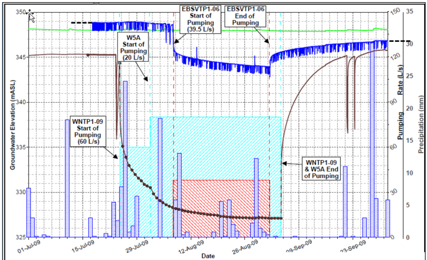
Figure 12. Water level record during WNTP1-09 pumping test
