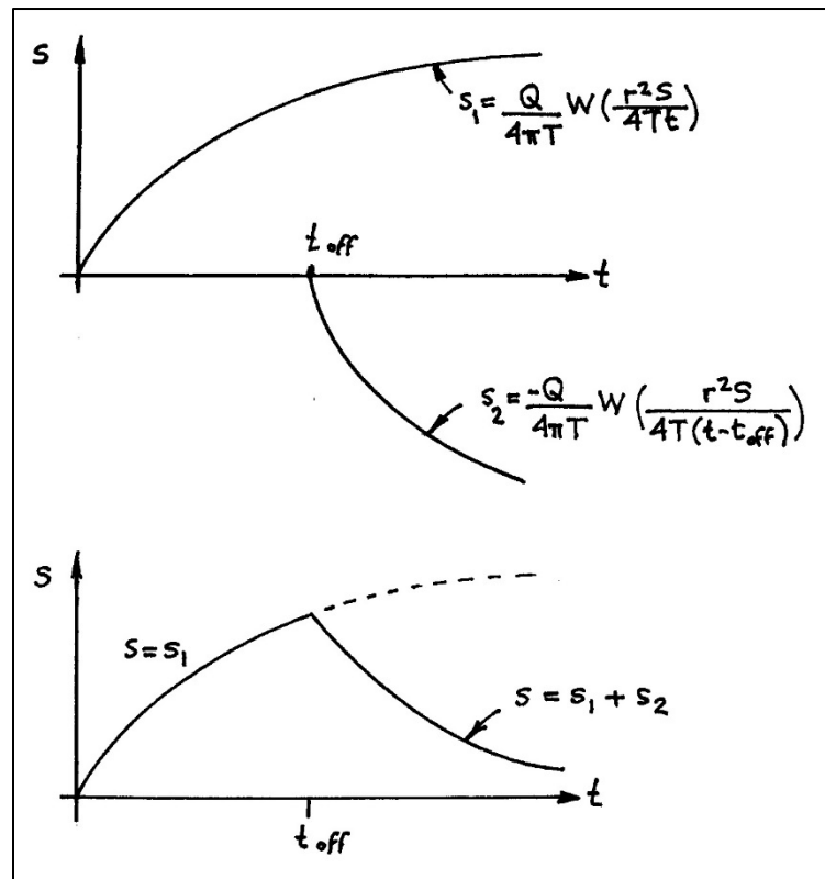
Figure 14. Application of the Theis (1935) solution for a finite duration of pumping
