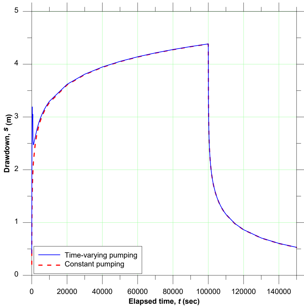
Figure 5. Complete drawdown record for the example
