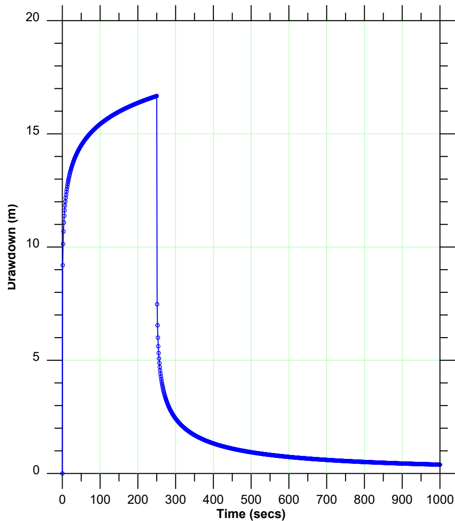
Figure 27. Calculated drawdowns during pumping and recovery
