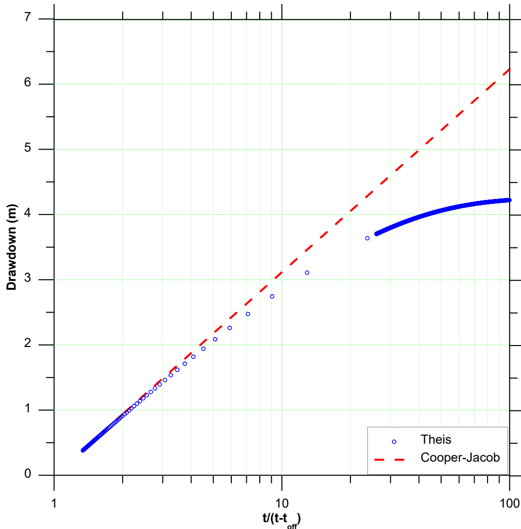
Figure 16. Theis solution and Cooper-Jacob solutions, semilog recovery plot
