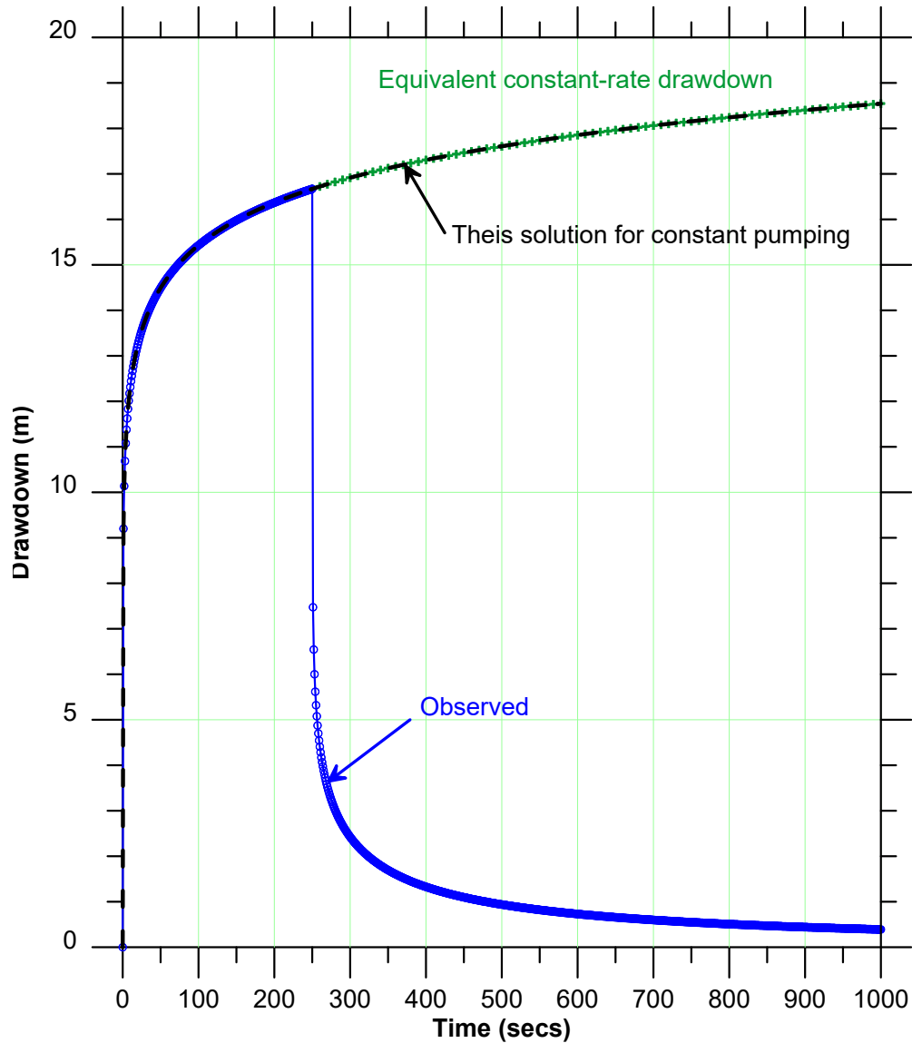
Figure 29. Actual drawdown and equivalent constant-rate drawdown
