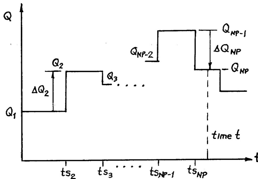
Figure 26. Discrete representation of an arbitrary pumping history
