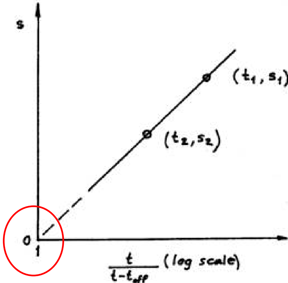
Figure 18. Asymptotic response for the straight-line recovery analysis
