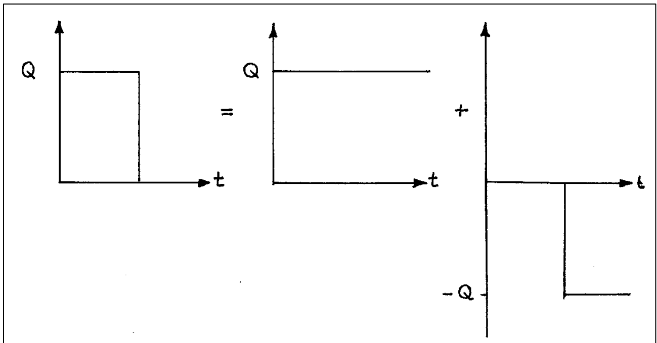
Figure 13. Illustration of superposition applied for a finite duration of pumping
