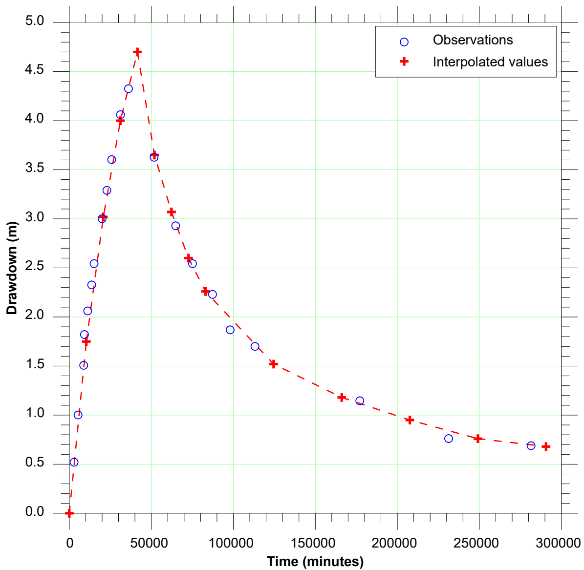
Figure 32. Raw drawdown data with interpolated values
