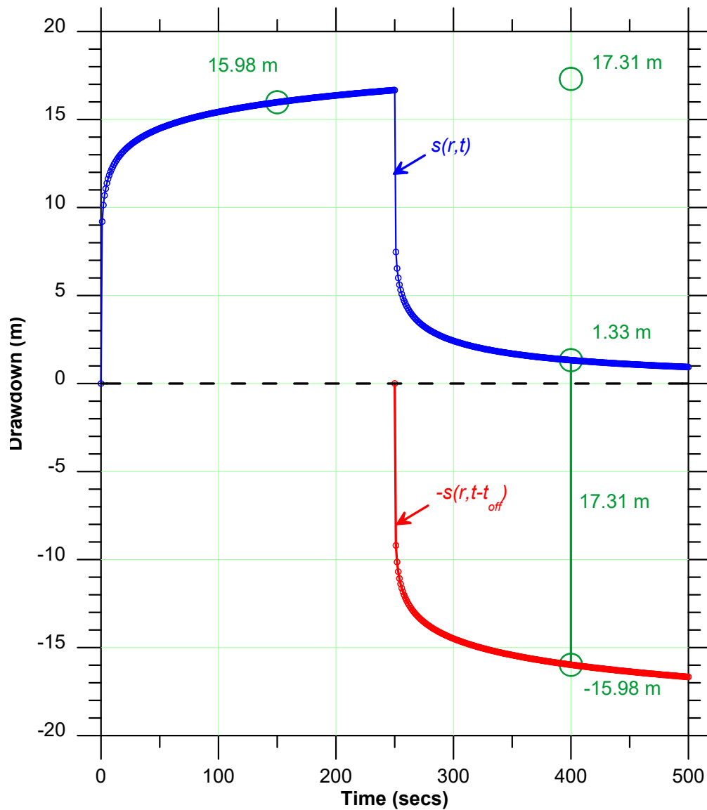
Figure 28. Calculation of the equivalent constant-rate drawdown at 400 seconds
