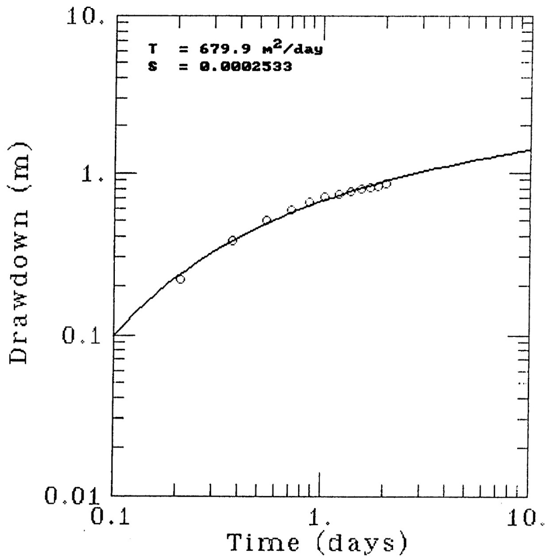
Figure 2. Analysis of the June 26, 1993 recovery data
