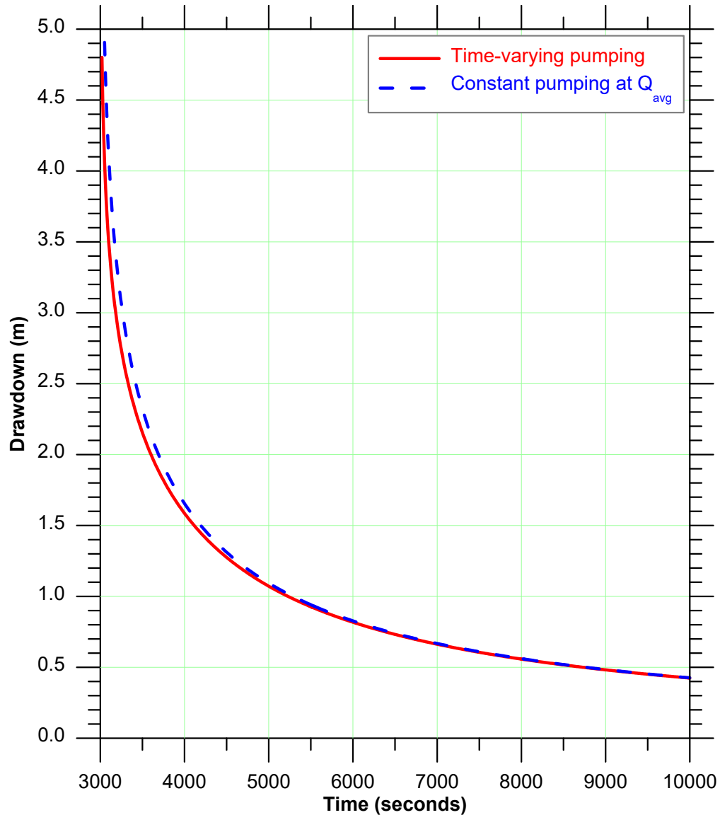
Figure 10. Comparison of recoveries for time-varying and constant pumping
