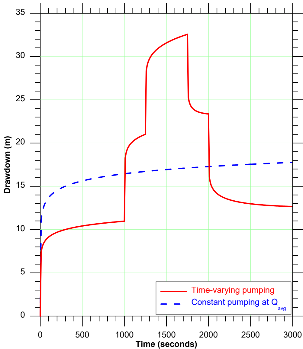
Figure 8. Comparison of drawdowns for time-varying and constant pumping
