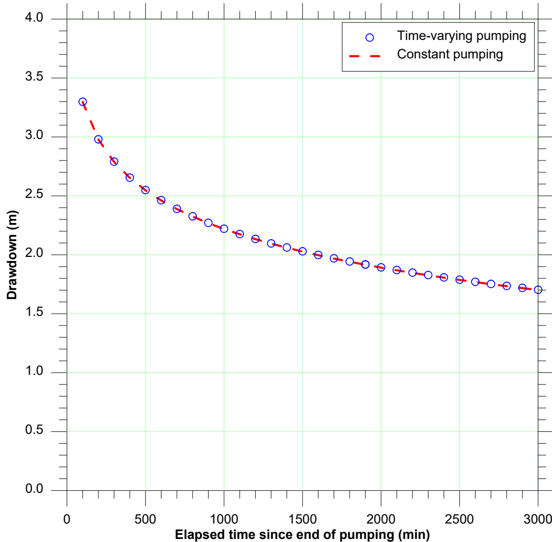
Figure 6. Drawdowns at r = 5 m following the end of pumping
