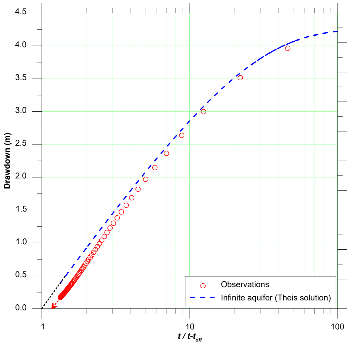
Figure 20. Recovery analysis for an aquifer with a zero-drawdown boundary
